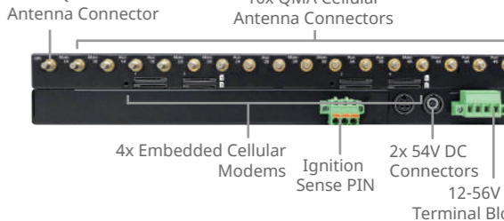
Back: 1x QMA GPS Antenna Connector, 16x QMA Cellular Antenna Connectors
