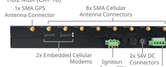
Back: 1x SMA GPS Antenna Connector, 8x SMA Cellular Antenna Connectors
